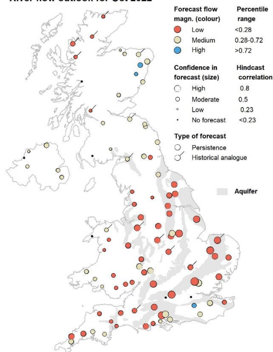
River flow outlook for Oct 2022
