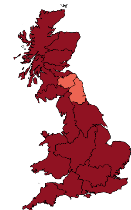
Lowest rainfall forecast
