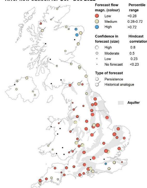
River flow outlook for Oct - Dec 2022
